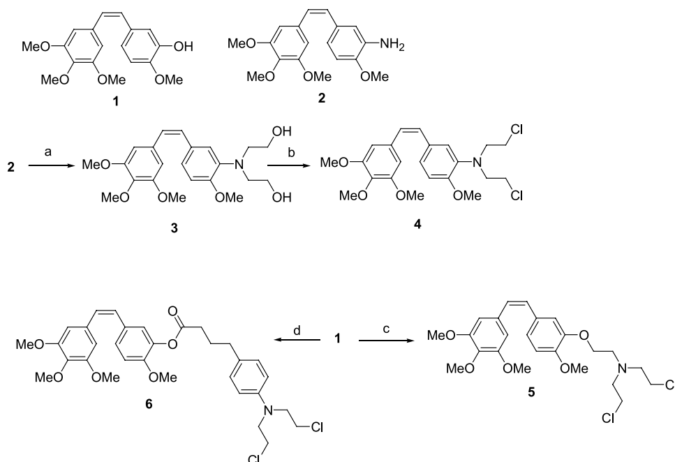
Scheme 1. Reagents and conditions: (a) CaCO 3 , 2-chloroethanol, water, reflux; (b) methansulfonyl chloride, TEA, DMF, rt. and then LiCl, 80°C; (c) tris(2-chloroethyl)amine, potassium tert -butylate, DMF, rt; (d) chlorambucil, EDCI, DMAP, CH 2 Cl 2 , rt.
