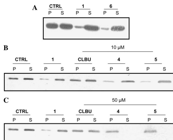
Figure 2. Inhibition of tubulin polymerization or depolymerization by combretastatin, chlorambucil, and their hybrids. P represents the pelletable fraction (polymerized tubulin) and S represents the soluble fraction (unpolymerized tubulin). Western blots are representative of at least three experiments that gave similar results.
